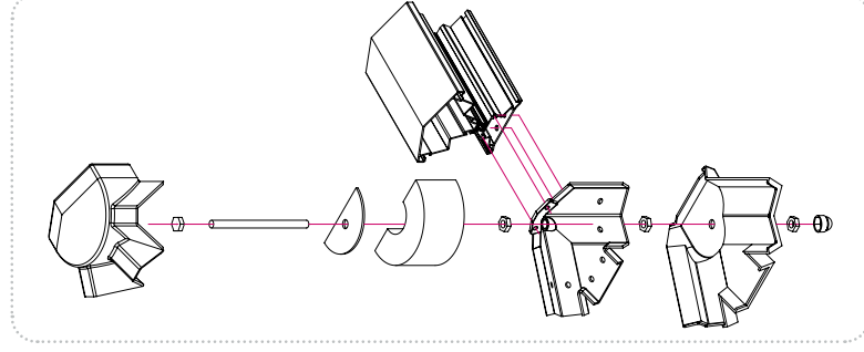
Spider bracket screws CRS 8626S CRS 9626S
